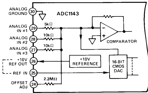
Figure 2. Analog Input Block Diagram
