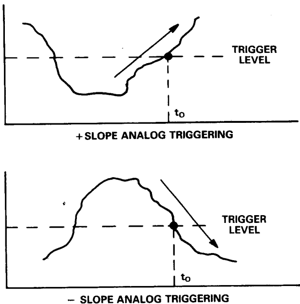
Figure 3. Analog Slope Triggering
