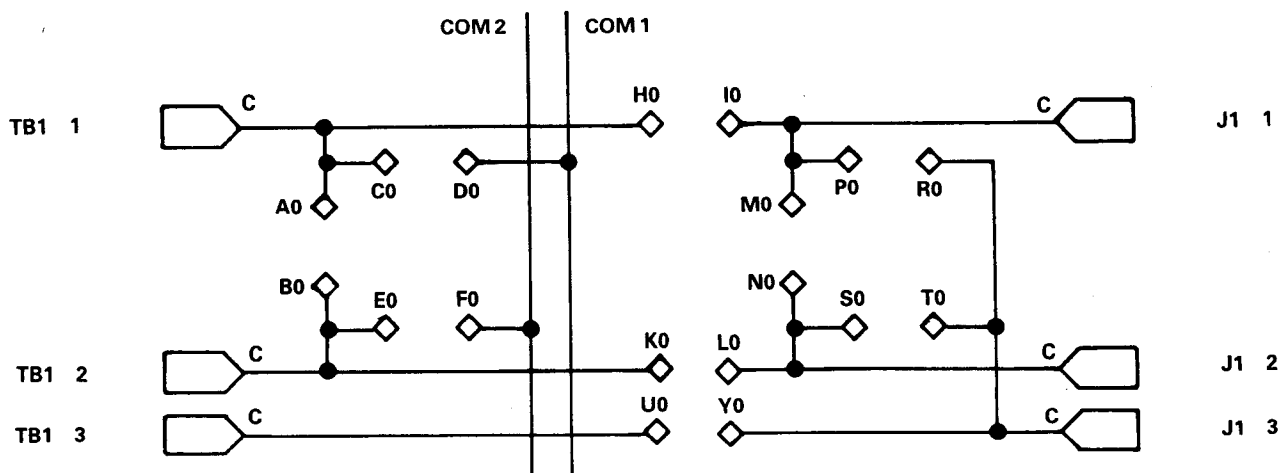
Figure 4. STB-GP Input Network
