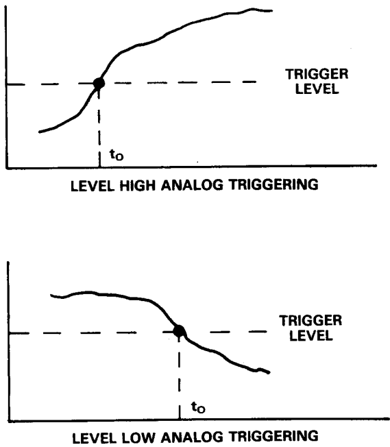
Figure 2. Analog Level Triggering
