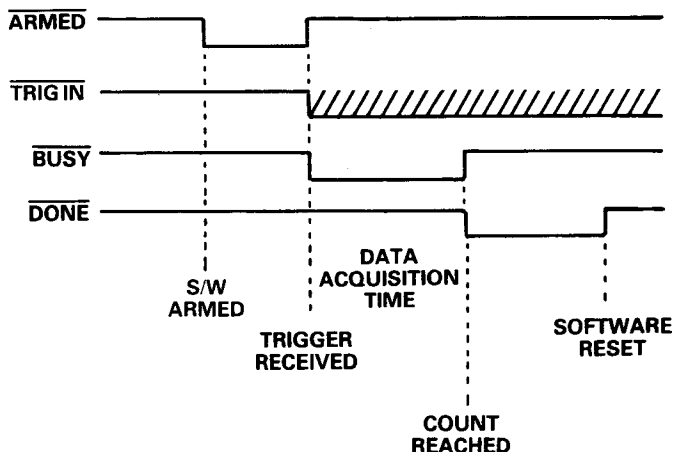
Figure 1. External TTL Triggering (Post Trigger Mode)
